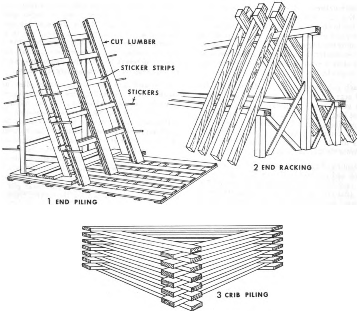
Figure 11-3. End, rack, and crib piling methods.
